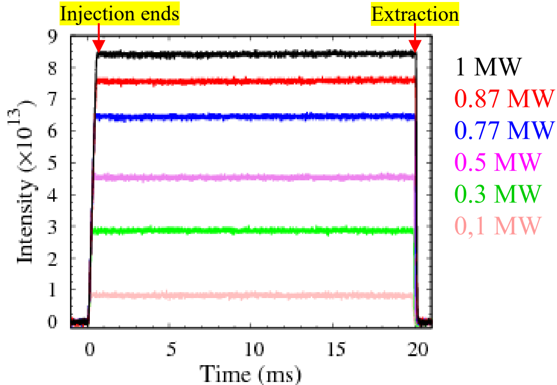
Circulating beam intensity measured by an SCT. There is no detectable intensity loss even at 1 MW.
