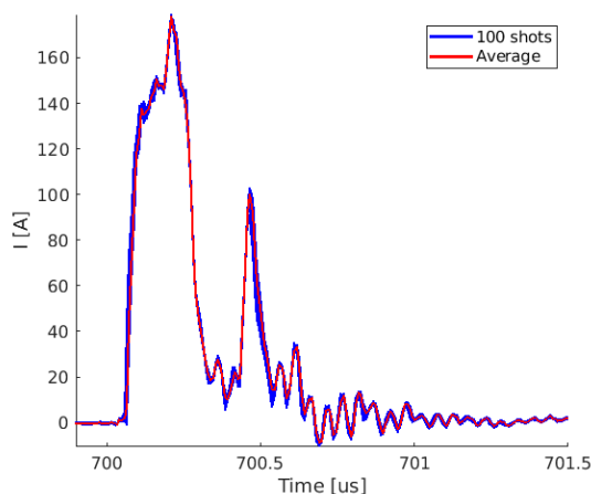
Figure 5: High-voltage current pulse profile measured on the high-voltage electrode side.
