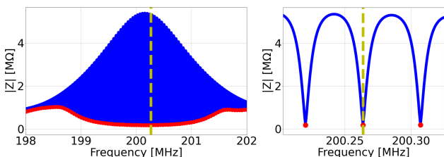
Figure 2: Left: impedance sum (blue) of the six SPS accelerating RF cavities damped with their OTDFB systems. The frequency resolution is \Delta f = f_0/50 . The red dots are the minima of the notches and represent the impedance sum with \Delta f = f_0 . The yellow line marks the design RF frequency at injection energy. Right: zoom around the RF frequency.
