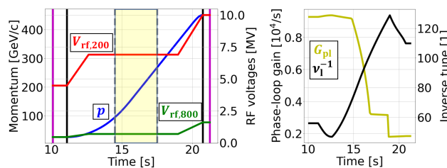
Figure 5: Left: momentum program (blue) together with the voltage programs of the 200 MHz (red) and 800 MHz (green) RF systems. The magenta (black) lines mark the start and the end of the simulations (ramp). The shaded area indicates the time interval for controlled emittance blow-up. Right: phase-loop gain (yellow) and number of turns per synchrotron period (black) along the cycle.
