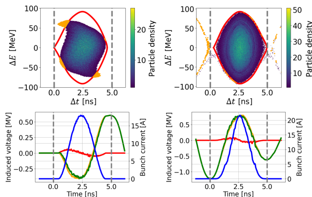
Figure 1: Top: distributions of bunch 1 at injection (left) and after 0.5 s (right). The particles marked in orange are outside the separatrix (red). Bottom: corresponding profiles (blue). The total induced voltage (green) is the sum of the induced voltage from the impedance model (orange) and the space-charge voltage (red). The grey lines mark the RF period.
