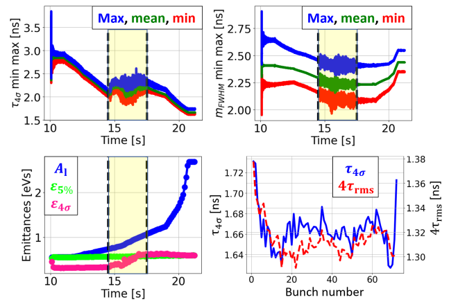
Figure 7: Top and bottom left: same color legends as in Fig. 6. The shaded area indicates the time interval for controlled emittance blow-up. Bottom right: extracted \tau_{4\sigma} (blue) and 4\tau_{\text{rms}} (red) along the batch.
