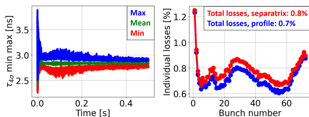
Figure 4: Evolution of maximum, mean and minimum \tau_{4\sigma} , out of 72 bunches. Right: losses along the batch at 0.5 s, either counting the particles outside the separatrix with respect to the injected intensity (red), or evaluating the decrease in bunch current relative to the injected current (blue). The total losses for the 72 bunches are reported in the legend.
