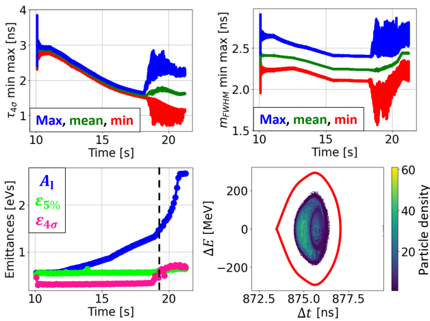
Figure 6: Top: evolution of maximum, mean and minimum \tau_{4\sigma} (left) and profile position (modulo the RF period) computed as middle point of FWHM (right), out of 72 bunches. Simulation without controlled emittance blow-up. Bottom left: bucket area (blue), \epsilon_{5\%} (green) and \epsilon_{4\sigma} (magenta) of bunch 36 along the cycle. The black line marks 19.2 s. Bottom right: phase-space distribution of bunch 36 at 19.2 s.
