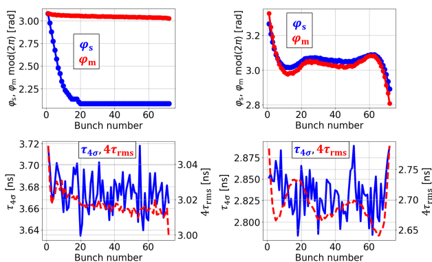
Figure 3: Top: average of the bunch profile (red) and synchronous phase (blue) along the batch at injection (left) and after 0.5 s (right). Bottom: \tau_{4\sigma} (blue) and 4\tau_{rms} (red) along the batch at injection (left) and after 0.5 s (right).
