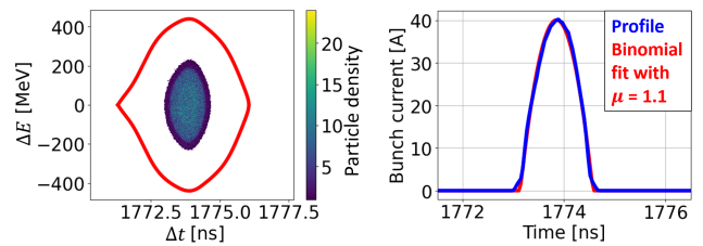
Figure 8: Distribution (left) and profile (right) of bunch 72 at extraction, applying controlled emittance blow-up as shown in Fig. 7. The binomial fit of the profile results in \mu = 1.1 .
