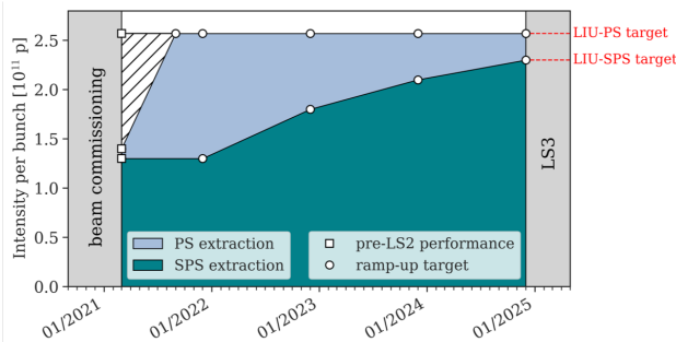
Figure 9: Planned bunch intensity ramp-up in the injectors until installation of HL-LHC.
