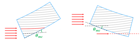
Figure 4: Impact conditions at a crystal collimator with negative (left) and positive (right) miscut angle.
