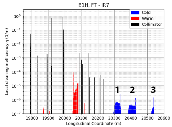
Figure 3: Simulated loss pattern in IR7 with protons for crystal collimation in operational configuration with no miscut on the horizontal plane of Beam 1 at 6.5 TeV.
