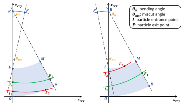
Figure 1: Geometrical model for negative (left) and positive (right) miscut in the reference frame of the bent crystal.
