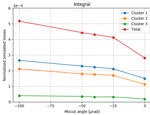
Figure 5: Integral of IR7-DS loss clusters in simulations for negative miscut angle values.
