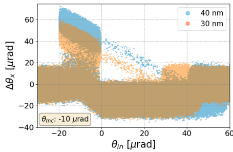
Figure 2: Simulated deflection resulting from a single passage of 450 GeV protons through a silicon crystal (4 mm length, 50 \mu\text{rad} bending) with impact parameters of 30 and 40 nm, as a function of the impact angle.
