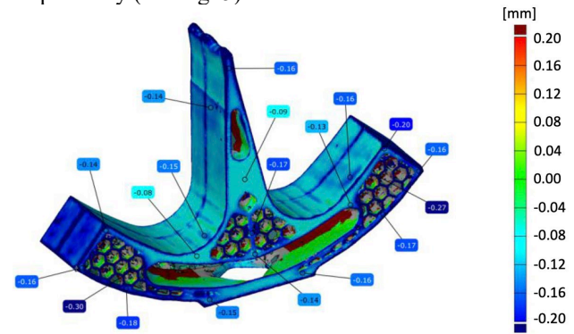
Figure 5: Measurements of 1/4 RFQ segment sample No1 - post-processed.
