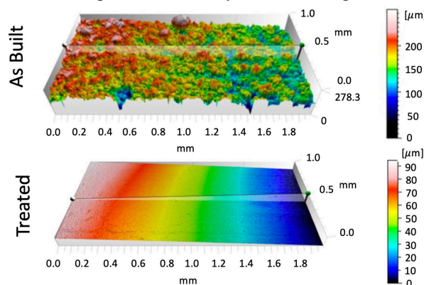
Figure 7: 3D surface roughness of the post-processed \frac{1}{4} RFQ sample.
