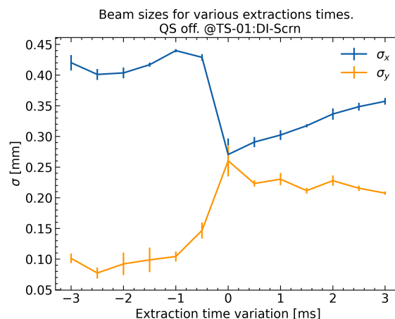
Figure 3: Fitted beam sizes at one YAG screen of the BTS for different stages in the TEE.
