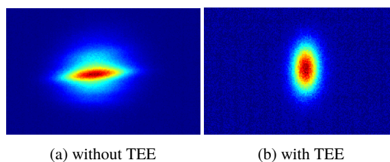
Figure 4: YAG screen beam images in the entrance of BTS, right after BO extraction.
