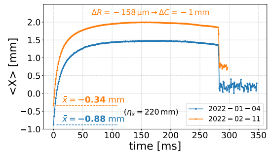
Figure 1: Effect of booster realignment on the average horizontal position. BPM acquisition at 1 kHz.
