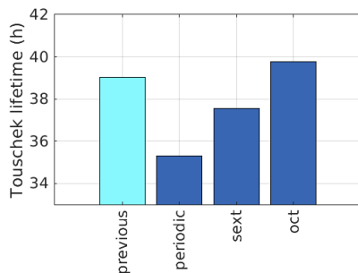
Figure 8: Touschek lifetimes at 200 mA in multi-bunch mode at 10 pm vertical emittance with sextupoles and octupoles setting from the previous run, periodic, after sextupoles optimization and after sextupoles and octupoles optimization.
