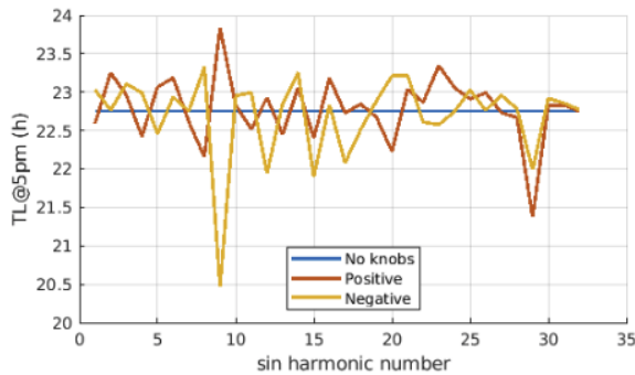
Figure 4: Effect of the sine wave octupolar knobs on the Touschek lifetime.
