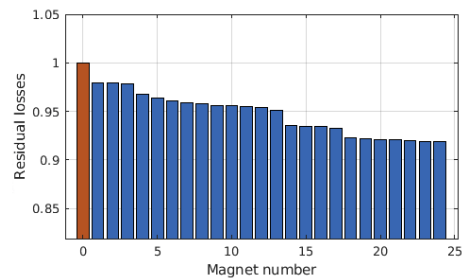
Figure 6: Fraction of total losses left after the optimization of 24 sextupole knobs. Total losses are reduced by about 8% at the end of the scan.
