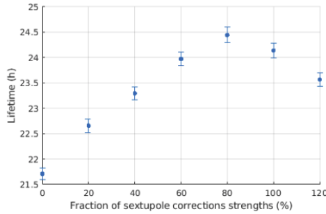
Figure 7: Scan of the amplitude of the previous run sextupole corrections before the new optimization. In this case, the best lifetime is with correctors at 80% of their initial value.
