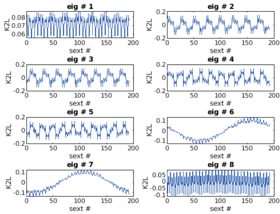
Figure 2: Sextupole pattern of the first 8 singular vectors.
