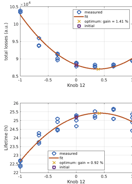
Figure 5: Scan of one sextupolar knob. The sum of the BLD signals (top plot) and the beam lifetime (bottom plot) as a function of the knob amplitude. The optimal value is the minimum of the parabola fitting the BLD data.
