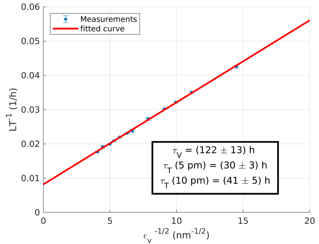
Figure 9: Touschek ( \tau_T ) and vacuum ( \tau_V ) lifetime measurement at 200 mA after the optimization.
