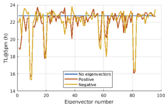
Figure 1: Effect of the off-energy optics correction singular vectors on the Touschek lifetime. The red and the yellow line are the lifetimes with a positive or negative knob applied to the sextupoles, the blue line is the lifetime without knobs.
