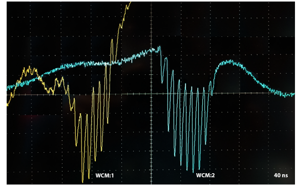
Figure 6: Wall current monitor signal at the HBT upstream (yellow) and downstream (green).
