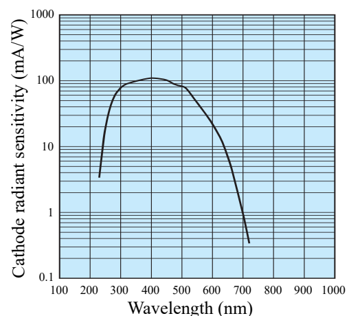
Figure 1: Cathode sensitivity for PMT [6].
