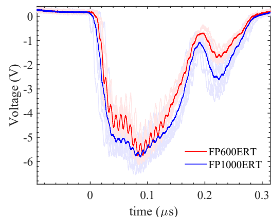
Figure 4: Signal comparison between different fiber types.
