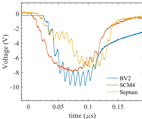
Figure 5: Beam loss measured at different places.
