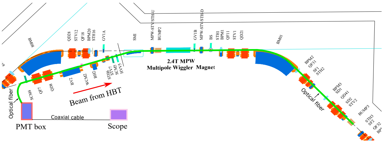
Figure 2: Schematic view of the optical fiber (green line) installation section.
