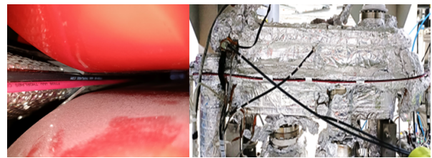
Figure 3: Optical fiber attached on the side of chamber through a quadrupole (left) and on a septum (right). Black and red cables are FP1000ERT and FP600ERT fiber respectively.
