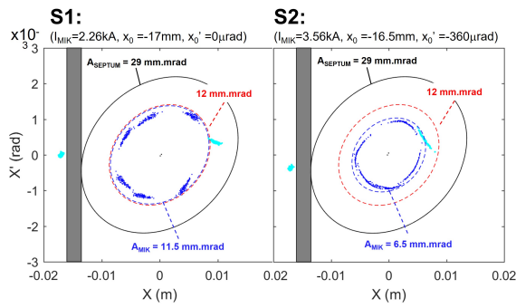
Figure 3: Horizontal phase-space at IP for two optimised solutions: (left) sole MIK current as parameter, (right) MIK current and injection parameters ( x_{inj} , x'_{inj} ) utilized.
