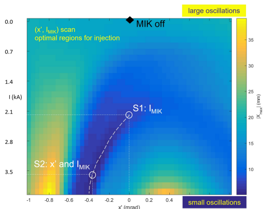
Figure 2: Injection angle and MIK current scan, identifying the best solutions in the (x'_{inj}, I_{MIK}) space in term of maximal residual oscillations over 7 turns. The dashed line guides the eye along the dark blue “valley” of minimum oscillations.
