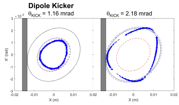
Figure 5: Resilience to DK excitation in the AT model. Left: DK angle at 1.16 mrad (standard injection value). Right: DK angle at 2.18 mrad, with the (x, x') phase-space at IP shaving the inner wall of the septum.
