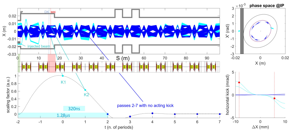
Figure 1: Beam dynamics of an on-crest bunch. Top-left: horizontal trajectories of the first two turns of the injected beam (cyan) with a full kick at injection and a second kick following the MIK time wave-form displayed in the bottom-left section. The following turns (dark blue) take place without MIK action. Top-right: representation of the same seven turn event in the (x, x') phase-space. Bottom-right: MIK field intensity function, showing the two kicking events, K1 and K2.
