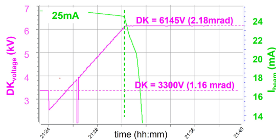
Figure 4: Machine test to verify its acceptance. Seven bunches for a total 25 mA beam (green trace) are probed with the DK at growing currents (pink trace). The I_{beam} sudden drop at 6.15 kV defines the acceptance of the ring.
