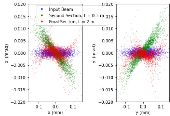
Figure 6: Horizontal and vertical phase space for the central of 11 longitudinal slices, at the end of the first vertical section, the final section, and initial phase space for this slice.
